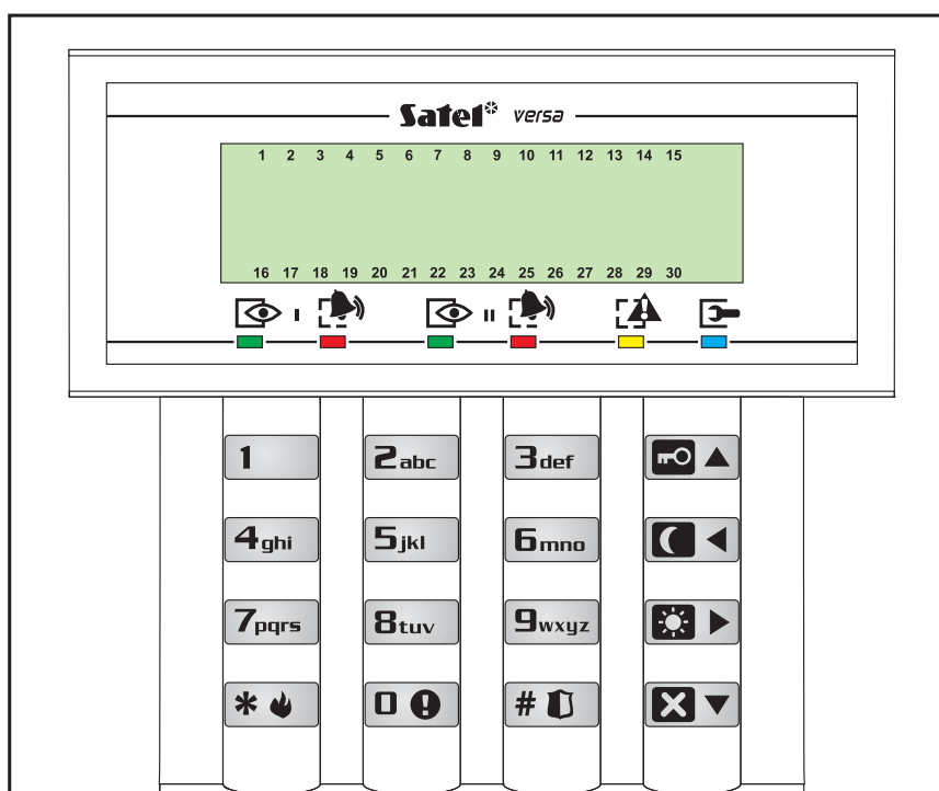
Rys. 1. Manipulator VERSA-LCD.
