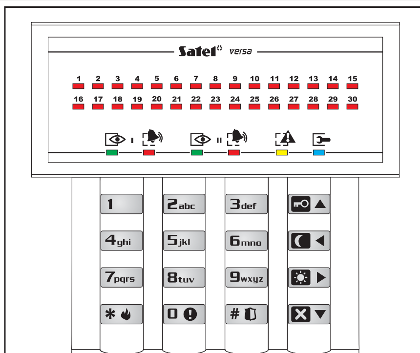
Rys. 2. Manipulator VERSA-LED.
